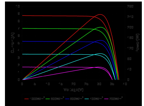
Current-Voltage and Power-Voltage Curves at Different Irradiances
